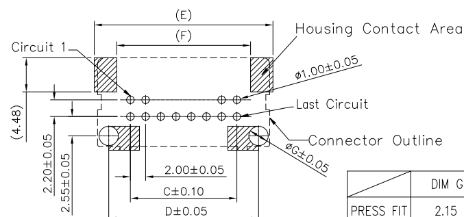
APPLICABLE P.C.B LAYOUT(REF.) P.C.B THICKNESS t=1.6mm
