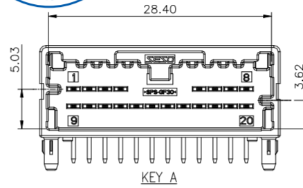
20PIN
