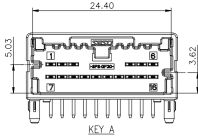
16PIN
