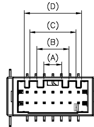
2*07~2*12 Pin
