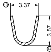
SECTION A-A SCALE 1:1 CONDUCTOR CRIMP 14/16 AWG
