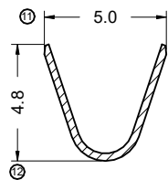
SECTION A-A SCALE 1:1 CONDUCTOR CRIMP 12 AWG
