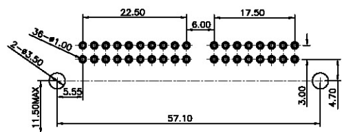
APPLICABLE P.C.B LAYOUT(REF.) P.C.B THICKNESS t=1.6mm
